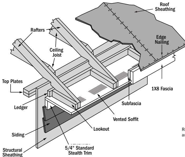
Rake System Installation Detail
