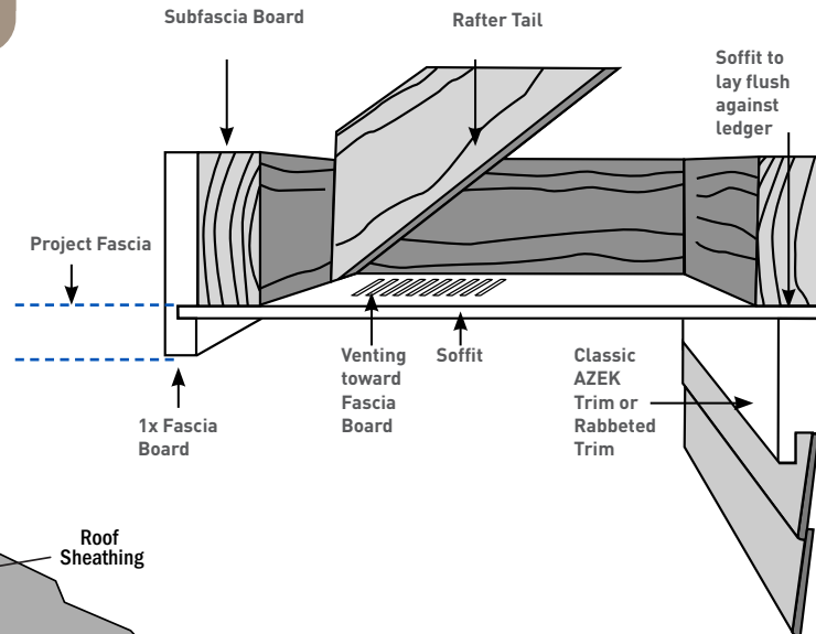
Additional Soffit System Installation Detail
